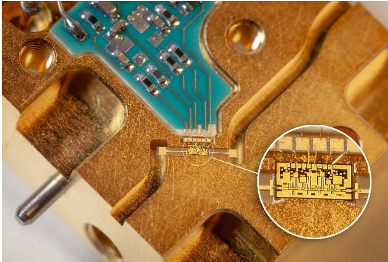
Close-up of the 89 GHz LNA MMIC integrated into the respective AWS microwave radiometer LNA module | © Fraunhofer IAF
