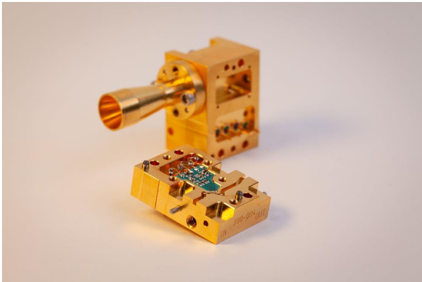
AWS microwave radiometer LNA module for the 89 GHz frequency range developed, manufactured and characterized at Fraunhofer IAF | © Fraunhofer IAF
